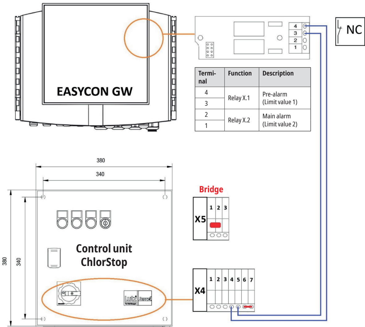
Fig. 4: Wiring of the control unit
