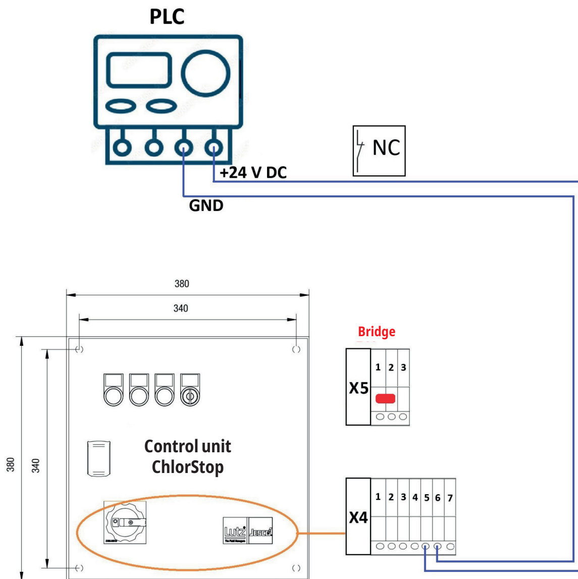
Fig. 5: Control via PLC with 24 V DC
