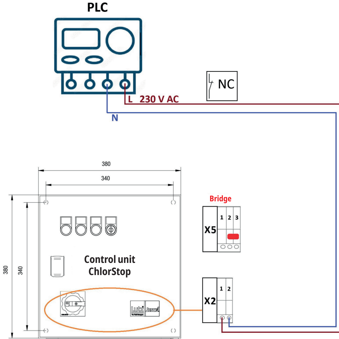
Fig. 6: Control via PLC with 230 V AC
