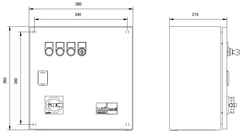
Fig. 3: Dimensional drawing
