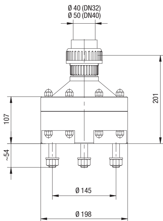
Fig. 3: Dimensional drawing
