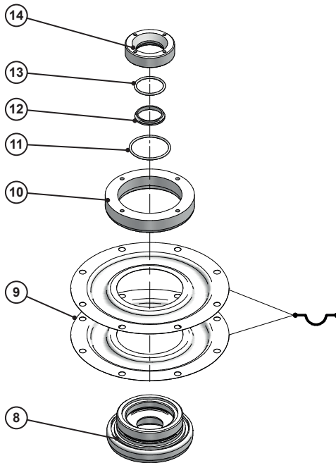
Fig. 6: Alignment of the diaphragm during installation
