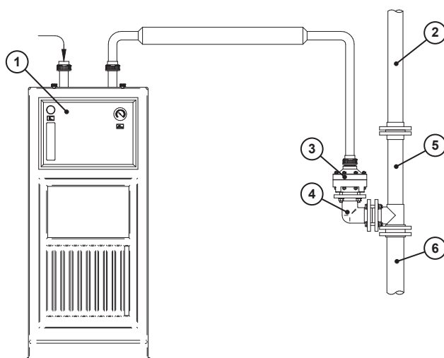
Fig. 5: Installation example
